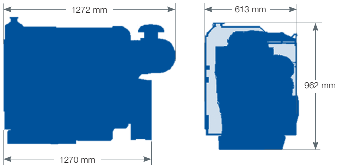
Engine package weights and dimensions
